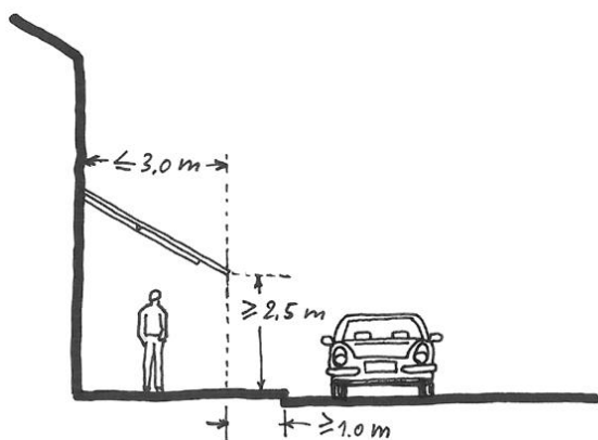
Figure 2 : Saillies mobiles
